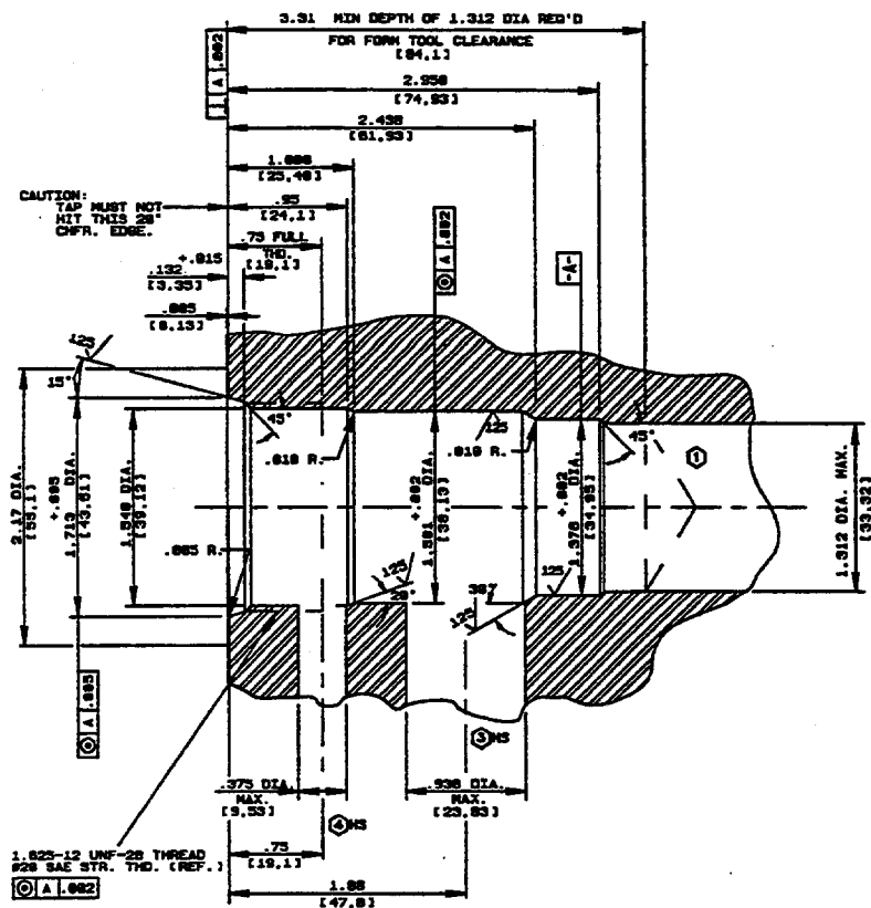
HS-1600-3 Form Tool
